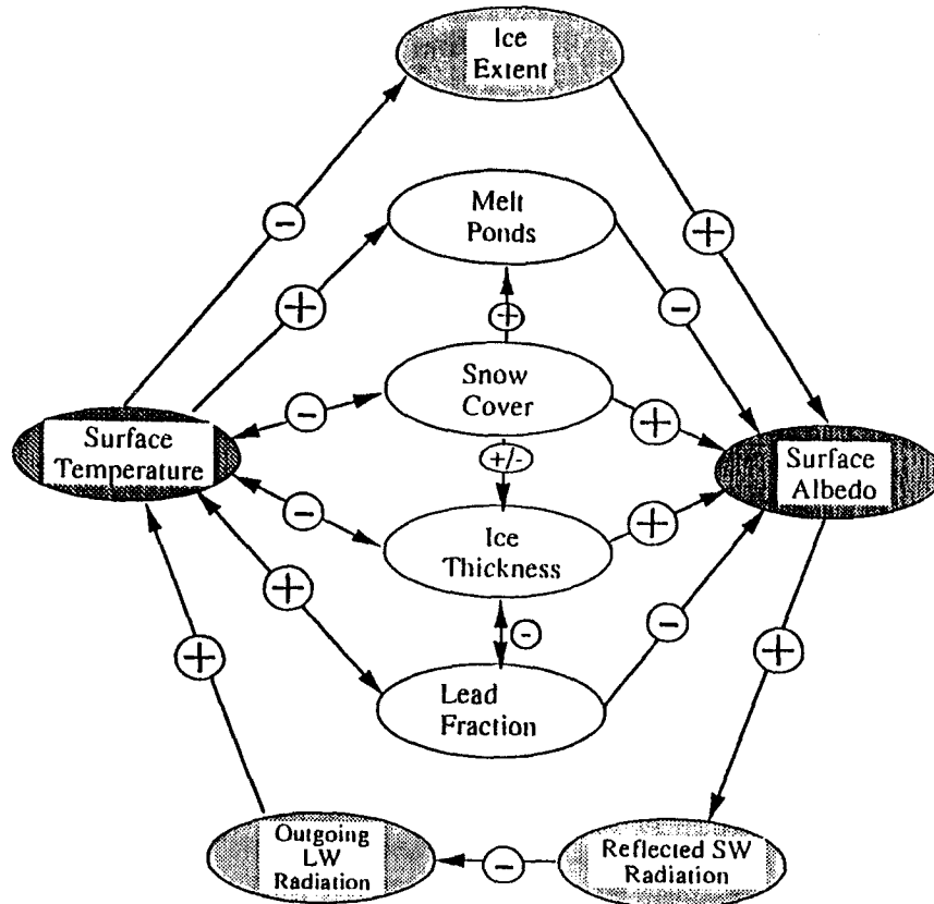
FIG. 11. Schematic diagram of the sea/ice-albedo feedback mechanism. The direction of the arrow indicates the direction of the interaction. A "+" indicates a positive interaction (an increase in the first quantity leads to an increase in the second quantity) and a "-" indicates a negative interaction (an increase in the first quantity leads to a decrease in the second quantity). A "+/-" indicates either that the sign of the interaction is uncertain or that the sign changes over the annual cycle.
