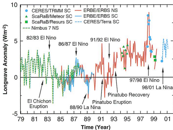
Fig. 1. Satellite record of tropical mean ( 20^\circ\text{S} to 20^\circ\text{N} latitude) anomalies in broadband thermal emitted LW flux. Anomalies are referenced to the ERBS scanner baseline period of 1985 through 1989, which most climate models use as a baseline for comparison (5). Results are shown from seven different broadband instruments on six spacecraft missions (6).
