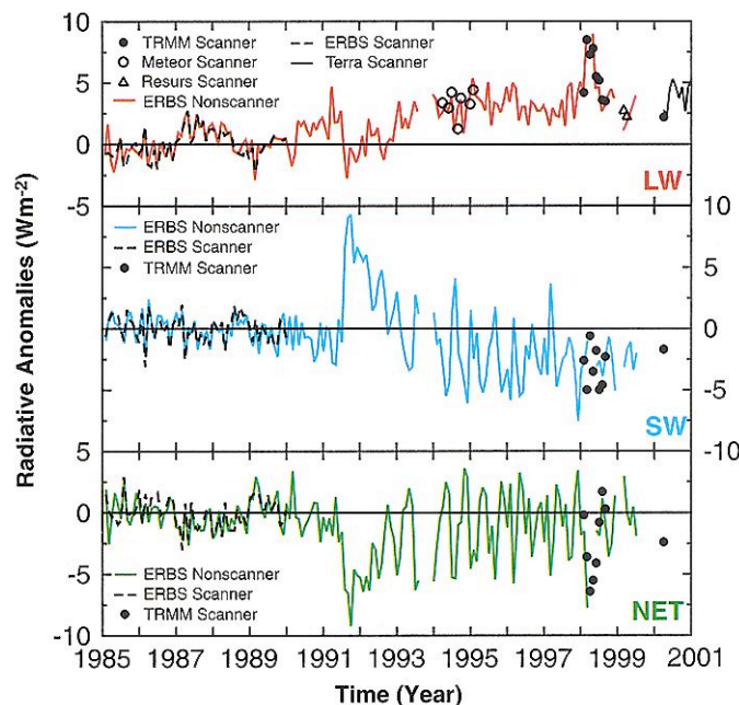
Fig. 2. Satellite record of tropical mean ( 20^\circ\text{S} to 20^\circ\text{N} latitude) anomalies in broadband thermal emitted LW flux, solar reflected SW flux, and net radiative flux. Net flux is defined as solar insolation – SW-reflected flux – LW-emitted flux. A smaller set of satellites is shown for SW- and net-radiative flux anomalies. Only those satellites whose orbits systematically sample the entire diurnal cycle in about a month, so the large diurnal cycle of solar reflected fluxes can be accurately determined across the entire tropics (25).
