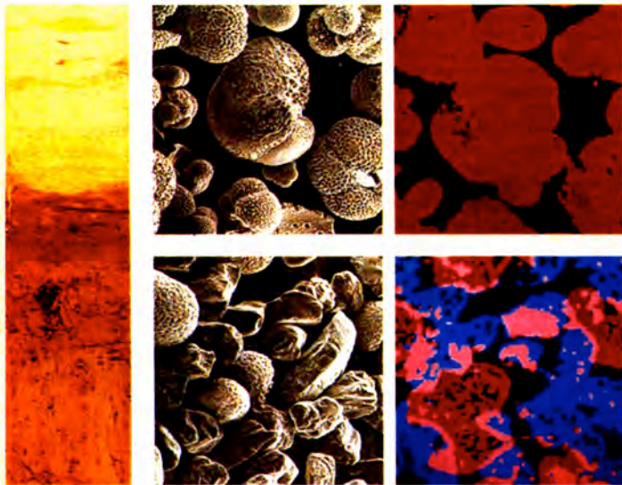
SEDIMENT CORE (left) from the North Atlantic testifies to an abrupt change in circulation at the end of the penultimate glaciation about 128,000 years ago. The transition (identified by Gerard C. Bond of Columbia University) spans a few millimeters and represents about 50 years. A scanning electron micrograph of coarse material from the dark sediments (bottom) reveals abundant rock fragments, rich in silicon (blue in an X-ray map), presumably dropped by melting icebergs. The light-colored sediments (top) include almost no rock and are made up mainly of shells, rich in calcium (red), from marine organisms that inhabit warm waters. (Shells in the dark sediments came from cold-water species.) The sudden revival of the Atlantic conveyor must have warmed the surface, eliminating icebergs and altering ecology.
