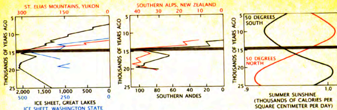
TIMING of glacial retreat was identical in the Northern Hemisphere (left) and in the Southern Hemisphere (center). The graphs give the extent of mountain glaciers and ice sheets from their source regions (in kilometers) and show that in ev-
