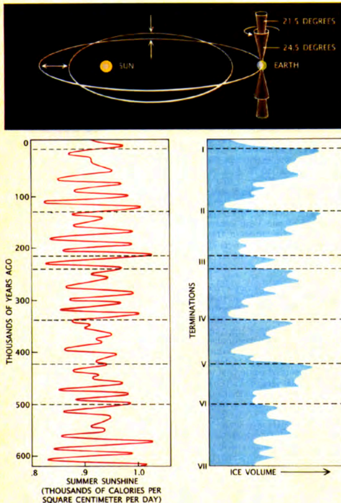
ASTRONOMICAL CYCLES (top) are the pacemaker of glaciation. The cycles—23,000 to 100,000 years in length—affect the eccentricity of the earth's orbit, the orientation of its spin axis (which slowly traces out a cone in space) and the tilt of the axis (which affects the width of the cone). The effect of the changes on the intensity of summer sunshine at high northern latitudes is shown at the left. The curve at the right indicates the volume of the earth's ice sheets, determined from isotopic studies of sea-floor sediments. Ice volume climbs gradually for about 100,000 years and then falls abruptly in ice-age terminations that correspond to episodes of increasing summer sunshine at northern latitudes. (Seasonality varies differently in the Southern Hemisphere, which suggests that northern seasonality must be what drives ice ages.)
