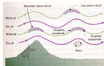
FIGURE 7.21 The formation of lenticular clouds.
